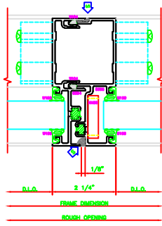
648 EXPANSION VERTICAL 9433 SHEARLOCK
