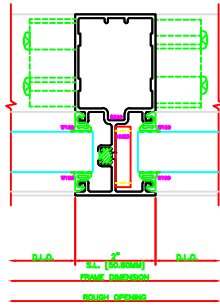
648 EXPANSION VERTICAL 9433 SHEARLOCK
